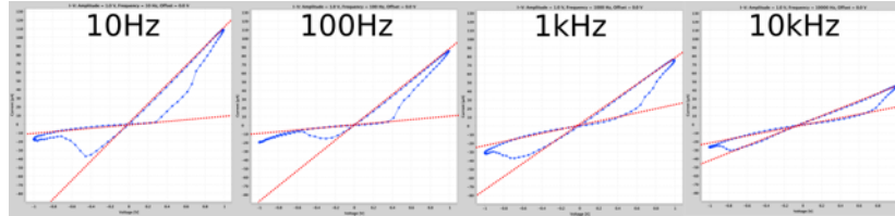
Figure 24: Comparison of 10Hz, 100Hz, 1kHz and 10kHz I-V plots of Tungsten memristor looking at the HRS and LRS in each case.
