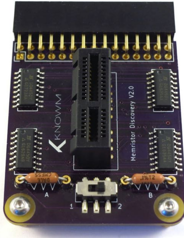
Figure 17: V2 Memristor Discovery Board
