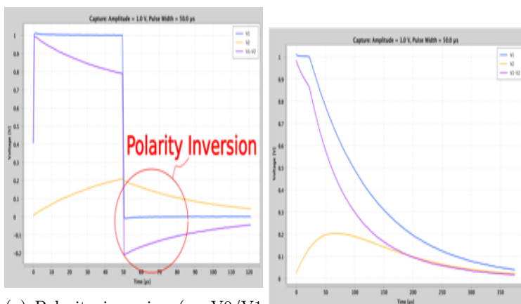
(a) Polarity inversion (on V0/V1 board) across memristor due to (b) Use of a 'long delay' pulse type charge accumulation on parasitic to mitigate polarity inversion with capacitance. high series resistance.
